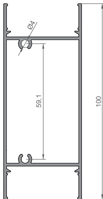
12010 DIVISOR 100
