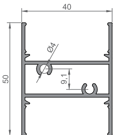
12007 Divisor peq. Abatible
