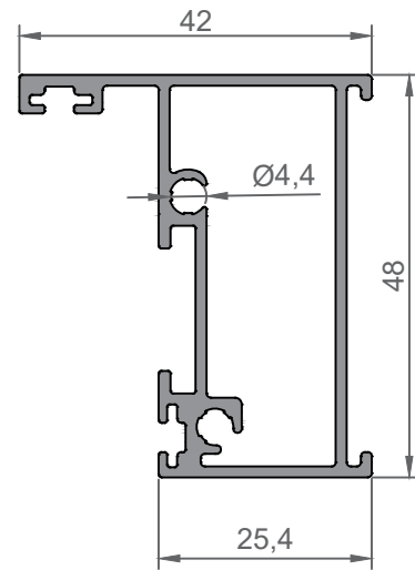
4655 MARCO LATERAL
