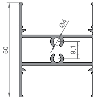
21/16007 Divisor peq. mallorq. Corredera
