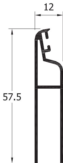
12006 Terminal lama grande mallorq.
