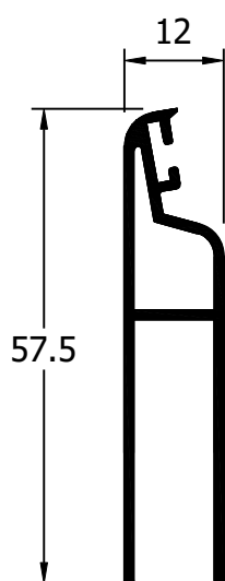
1200 Terminal lama grande mallorq.
