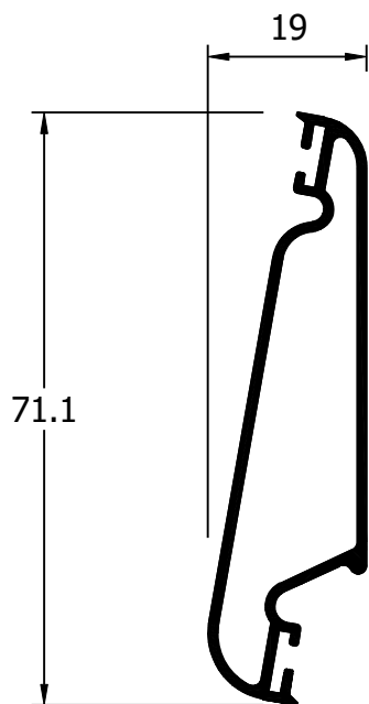
12002 Lama regulable mallorq.
