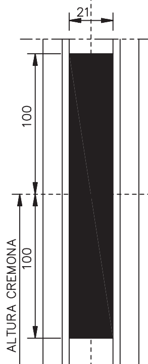
KIT CIERRE
