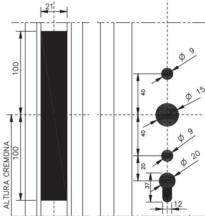
KIT CIERRE
