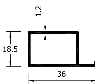
11030 Premarco 36x18.5 mm
