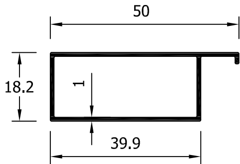
20046 Premarco 50x18.2 mm
